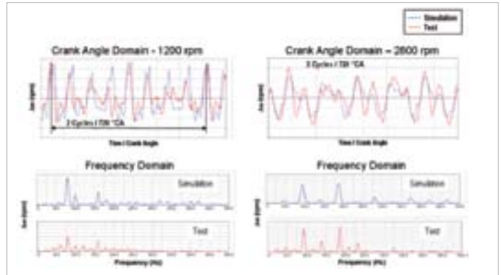
Figure 6: Correlation of Crank Nose Speed Fluctuation
