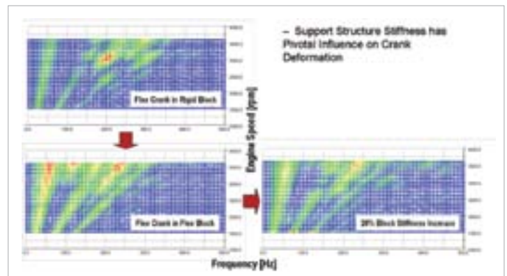
Figure 2: Support Structure Sensitivity, Influence on Crank Bending
