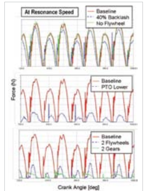
Figure 4: Selected Solutions of the Gear Resonance Mitigation Study
