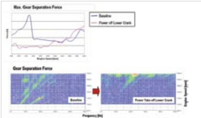
Figure 5: Solution for Gear Resonance: Power Take-off Moved to Lower Crankshaft
