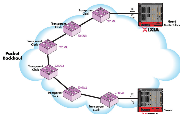
Figure 13. Test Setup: transparent clock correction field validation
