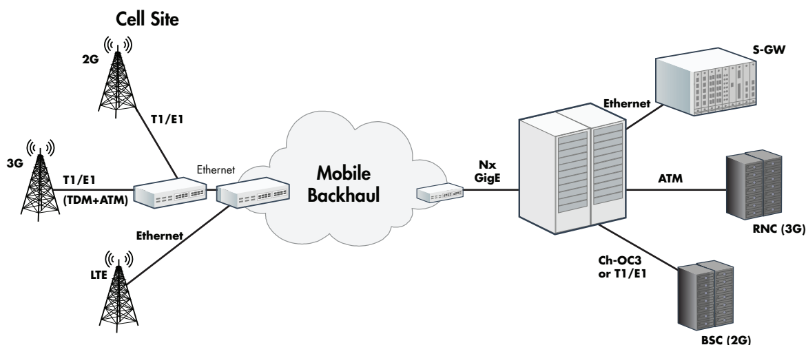
Figure 1. Mobile Backhaul Network
