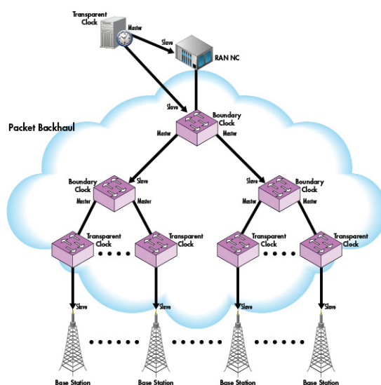
Figure 3. Timing over Packet using 1588v2
