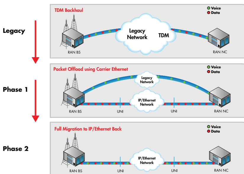
Figure 2. Mobile Backhaul Migration
