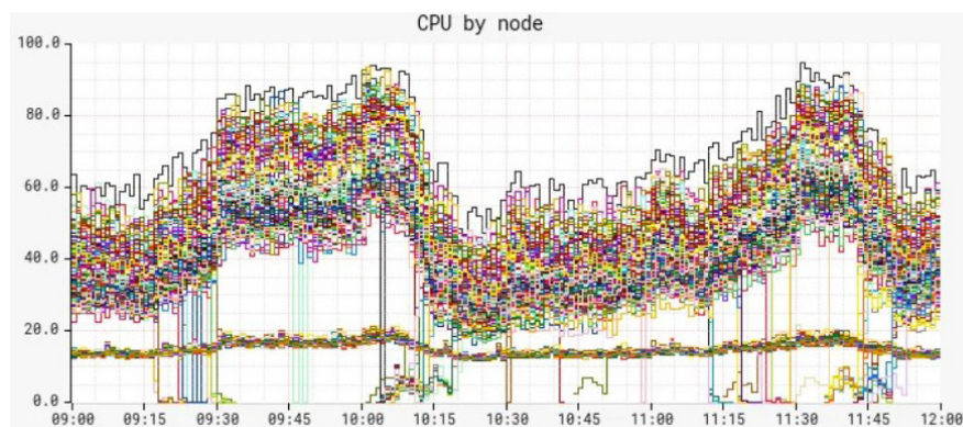
Figure 1. The graph illustrates the breakdown of CPU by node. While the analysis found roughly equal traffic distribution between nodes, CPU metrics demonstrated different bimodal distribution patterns. 1
