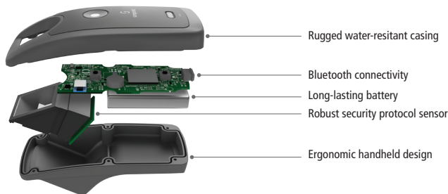
Figure 2: The Simprints Fingerprint Scanner
